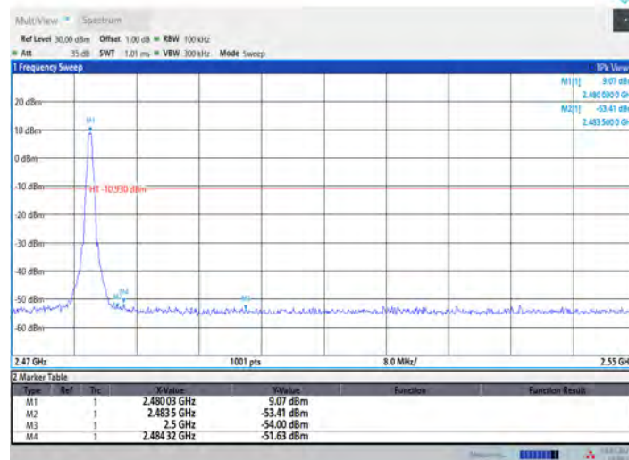
DH5_Ant7_High_2480
