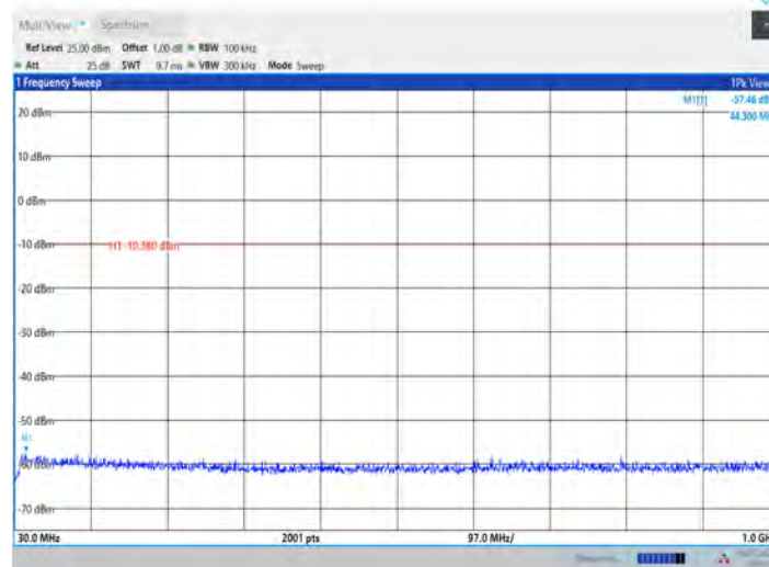
DH5_Ant7_2402_30-1000
