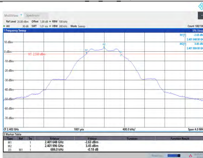
BLE_1M_Ant7_2402
