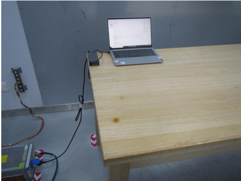
Conducted Disturbance
