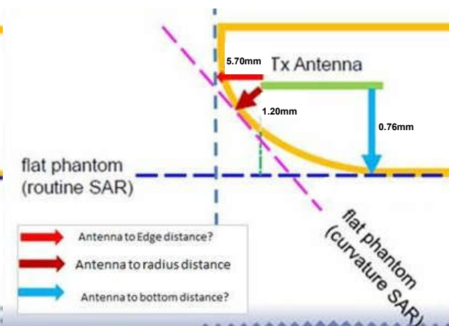
X=5.70mm, Y=0.76mm, Z=1.20mm Exterior Radius Dimension for WLAN
