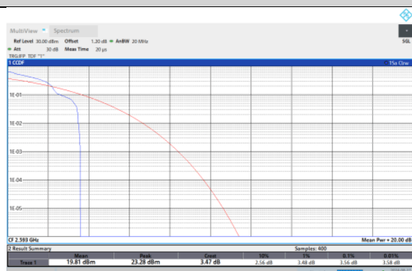
Band41-15MHz-64QAM-41515-1RB#0
