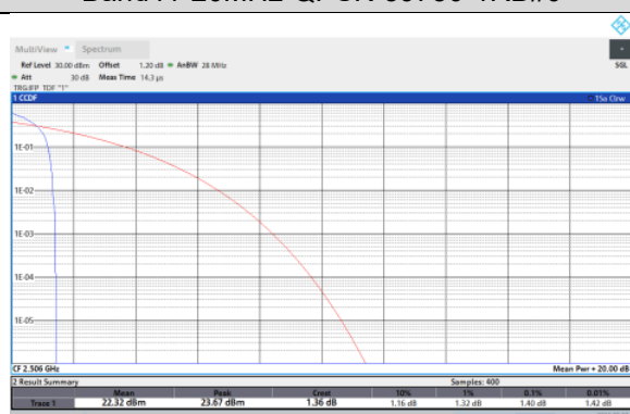
Band41-20MHz-QPSK-40620-1RB#0
