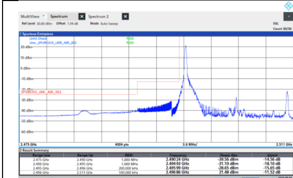
Band41-15MHz-16QAM-41515-1RB#74
