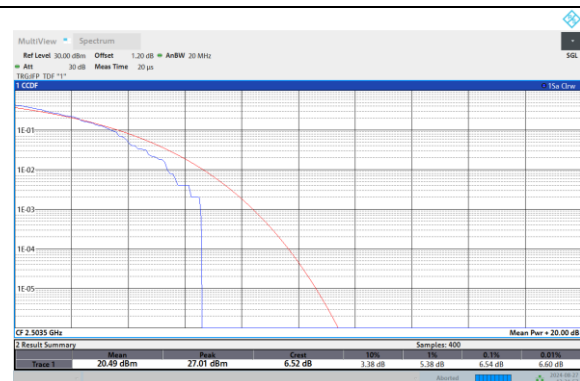
Band41-15MHz-64QAM-40620-75RB#0
