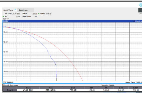
Band41-15MHz-16QAM-41515-75RB#0
