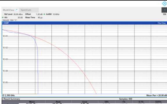
Band41-10MHz-QPSK-41540-1RB#0
