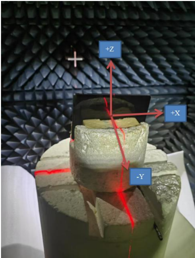
Fig.5. The DUT in the fully anechoic chamber
