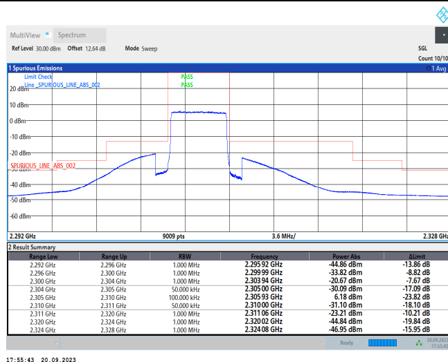
Band30-5MHz-QPSK-27685-25RB#0
