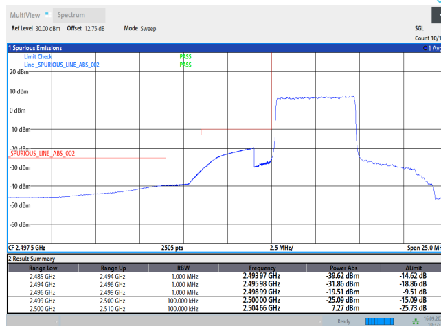
Band7-5MHz-QPSK-20775-25RB#0
