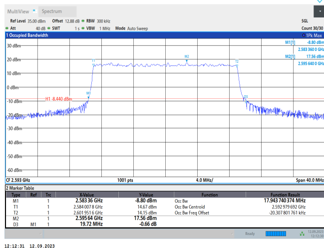
Band41-20MHz-QPSK-40620-100RB#0
