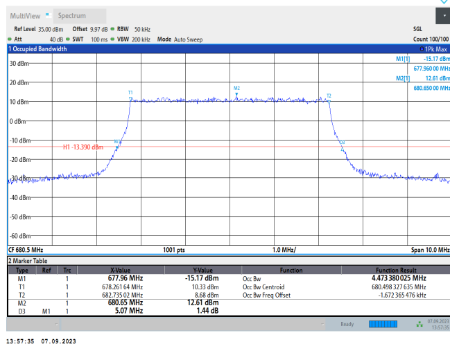
Band71-5MHz-16QAM-133297-25RB#0
