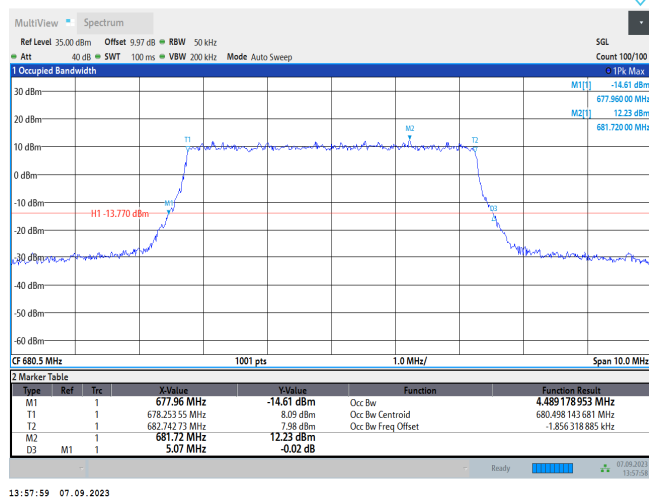
Band71-5MHz-64QAM-133297-25RB#0
