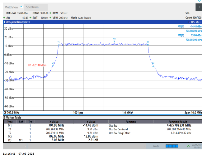
Band12-5MHz-QPSK-23095-25RB#0
