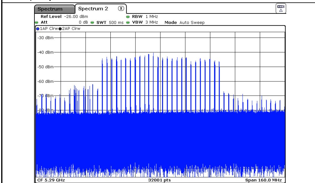
EUT (Client ) links with master on 5290MHz
