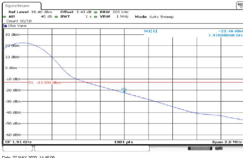
Band2-15MHz-QPSK-19125-75RB#0
