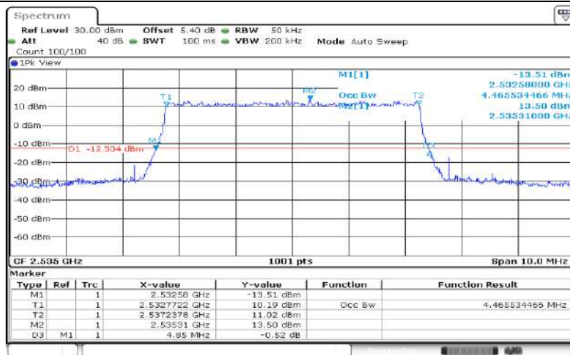
Band7-5MHz-QPSK-21100-25RB#0-4.466
