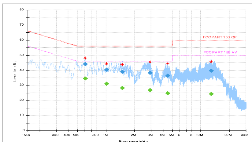
Full Spectrum
