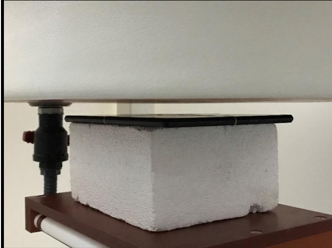
Rear Face of EUT with 0.9cm Gap
