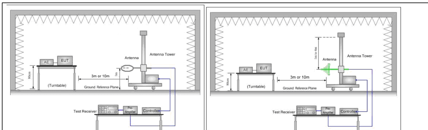
Figure 1. Below 30MHz
