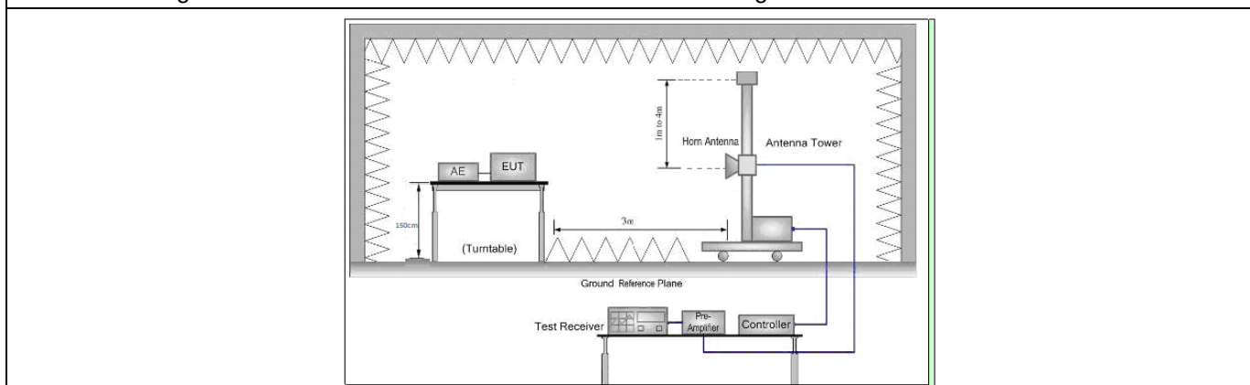
Figure 3. Above 1 GHz
