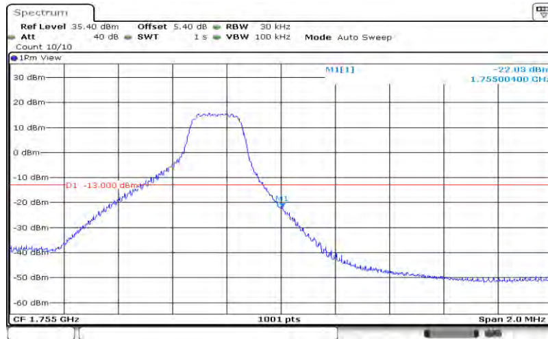
Band4-3MHz-16QAM-20385-15RB#0
