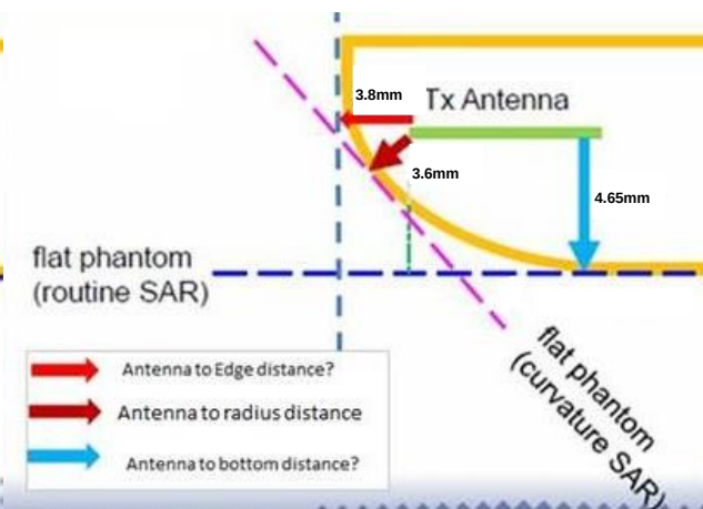
Curved Surface of Edge1, Test Separation 0 mm
