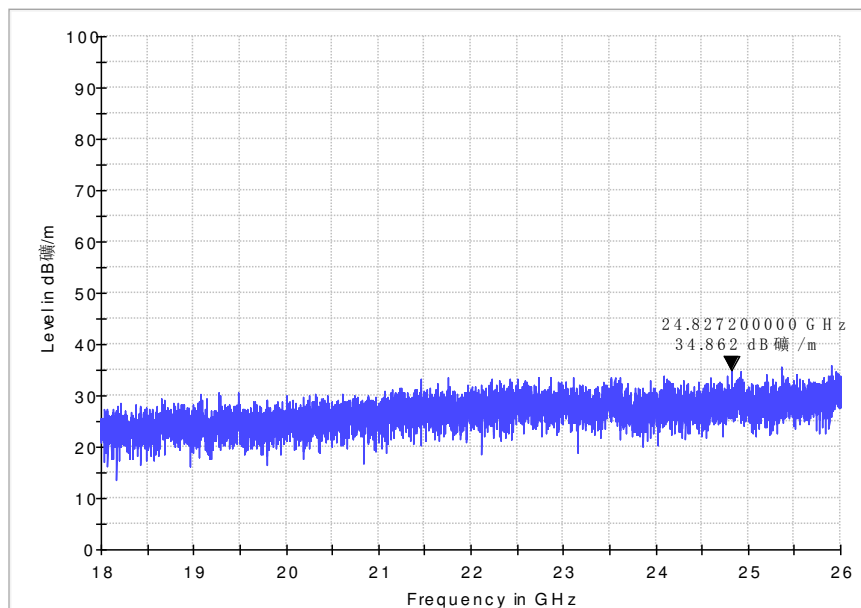
Fig 77. Radiated Spurious Emission (802.11b,ch1,18GHz~26GHz)
