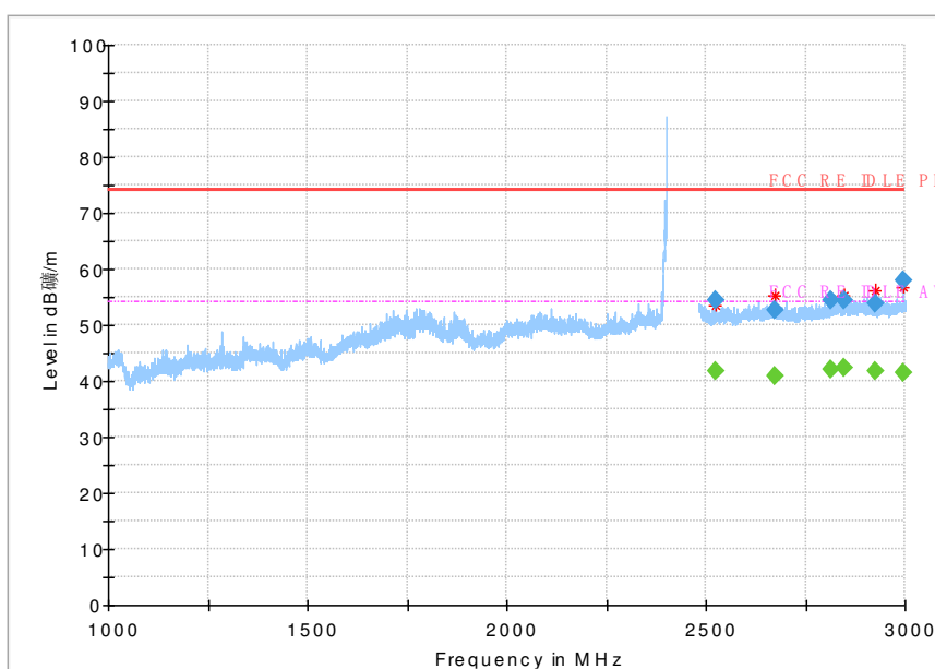
Fig 65. Radiated Spurious Emission (802.11g,Ch1,1GHz~3GHz)
