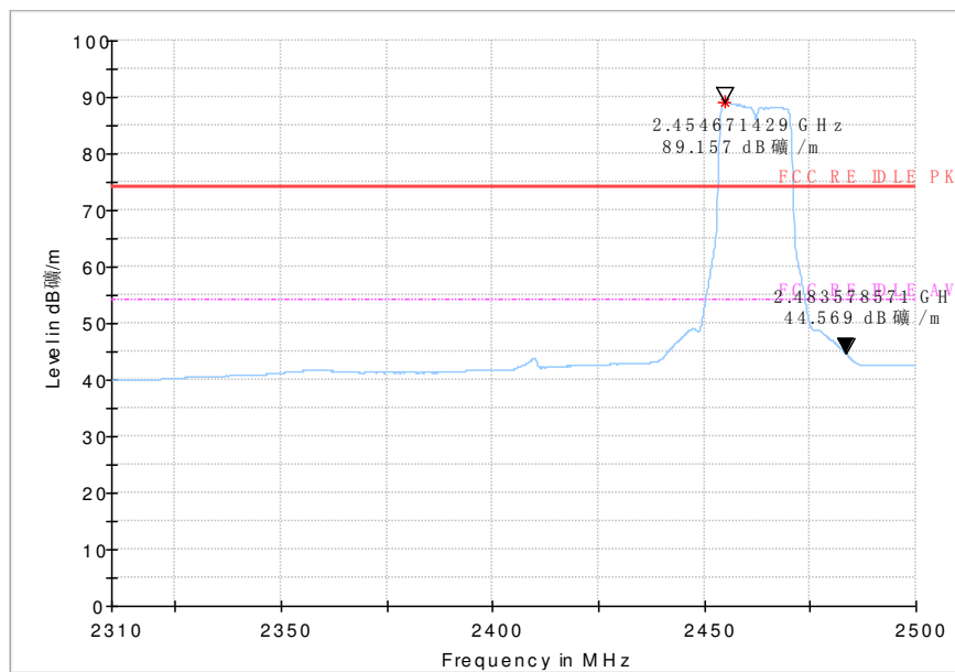
Fig 68. Radiated emission (Power): 802.11n (20M) , high channel
