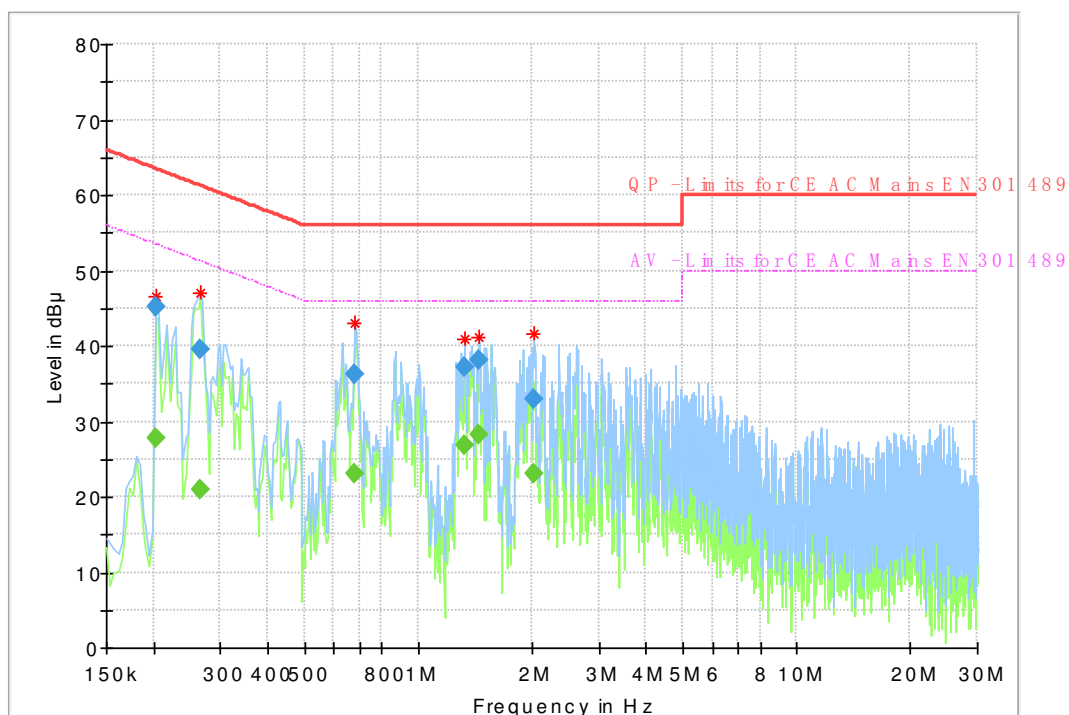
Fig 78. AC Powerline Conducted Emission
