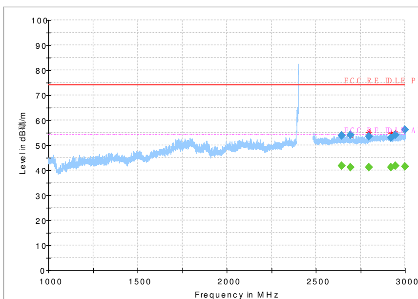
Fig 75. Radiated Spurious Emission (802.11 n-40MHz,Ch1,1GHz~3GHz)
