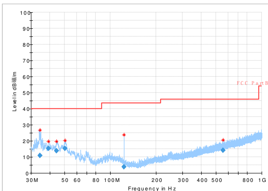
Fig 59. Radiated Spurious Emission (802.11b,Ch1,30MHz~1GHz)
