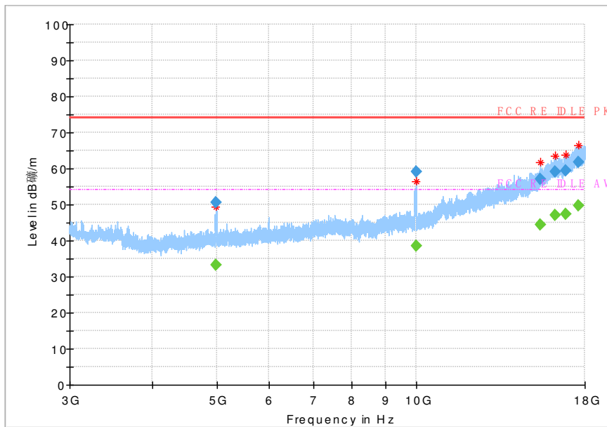
Fig 76. Radiated Spurious Emission (802.11 n-40MHz,Ch1,3GHz~18GHz)
