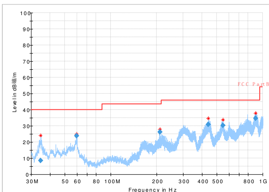
Fig 64. Radiated Spurious Emission (802.11g,Ch1,30MHz~1GHz)
