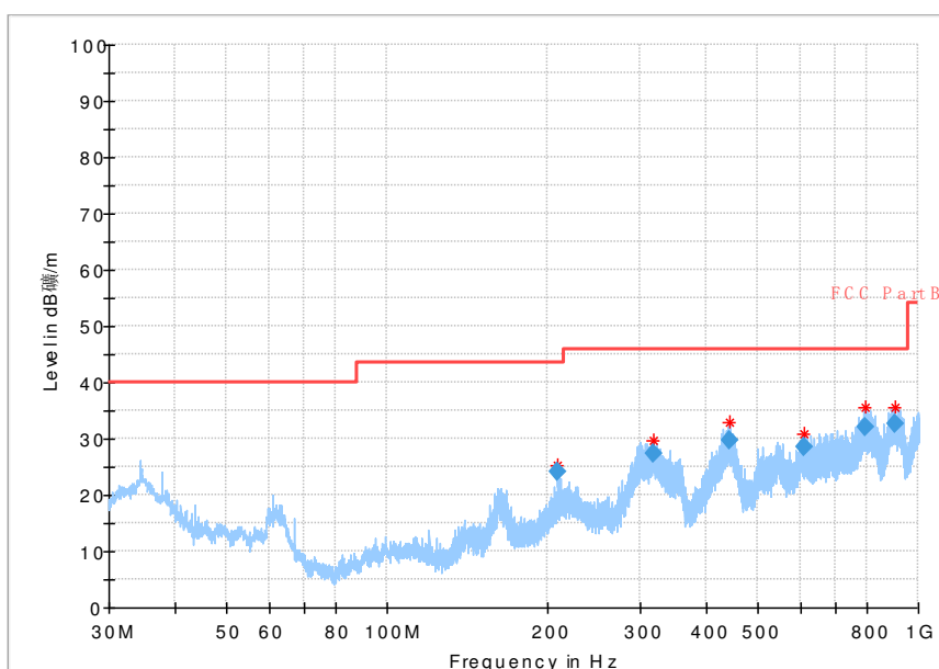
Fig 74. Radiated Spurious Emission (802.11 n-40MHz,Ch1,30MHz~1GHz)
