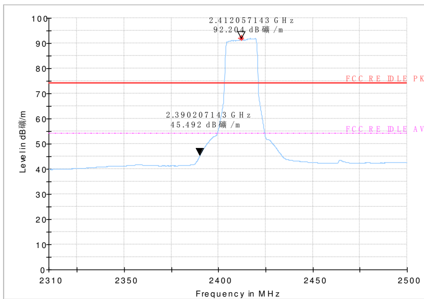
Fig 67. Radiated emission (Power): 802.11n (20M) , low channel
