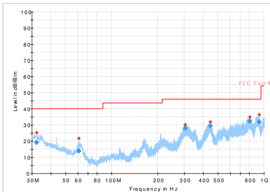
Fig 69. Radiated Spurious Emission (802.11 n-20MHz,Ch1,30MHz~1GHz)
