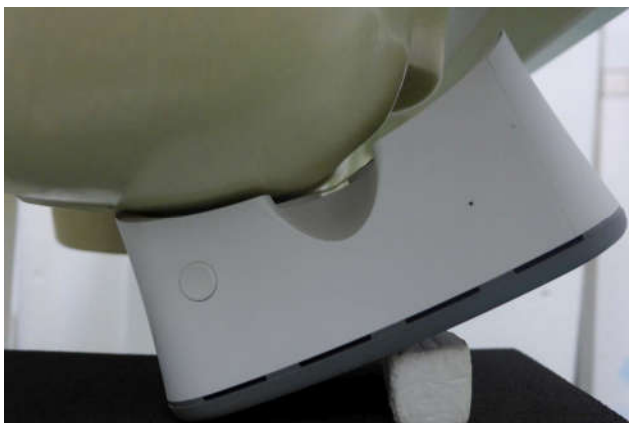
Near to Head (For Ant.2), Test Separation 0 mm
