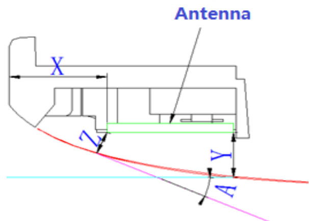
X= 4.14 mm, Y= 2.44 mm, Z= 1.07 mm The device exterior radius dimension
