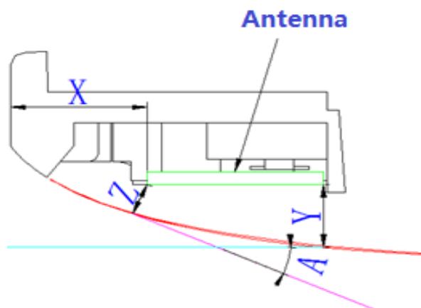
X= 4.14 mm, Y= 2.44 mm, Z= 1.07 mm The device exterior radius dimension
