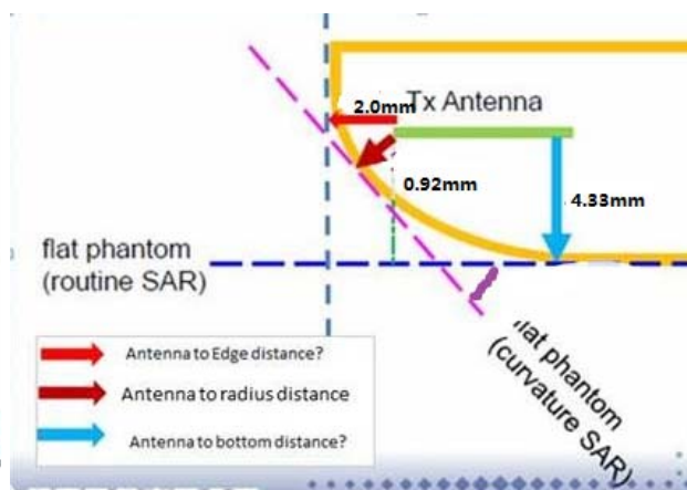
X=2.0mm, Y=4.33mm, Z=0.92mm Exterior Radius Dimension for WLAN
