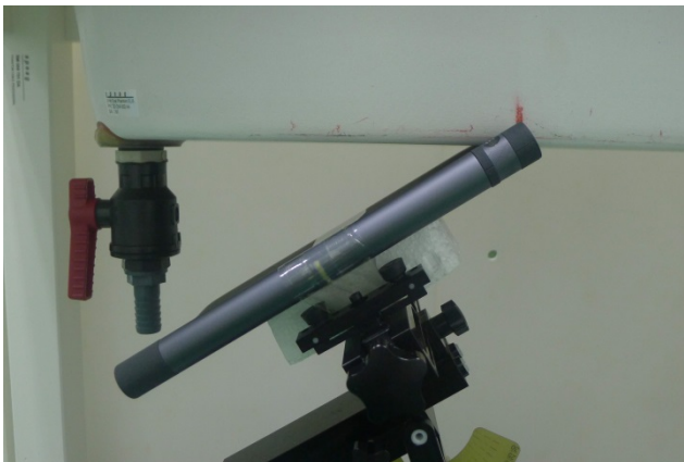
Bottom Face Edge 1_35 Degree, Test Separation 0 cm
