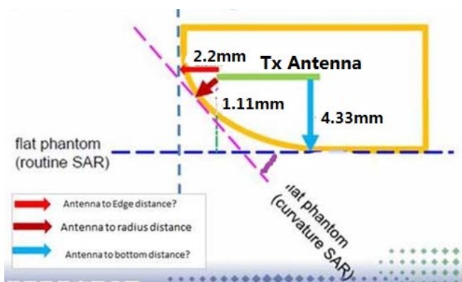
X=2.2mm, Y=4.33mm, Z=1.11mm Exterior Radius Dimension for WWAN
