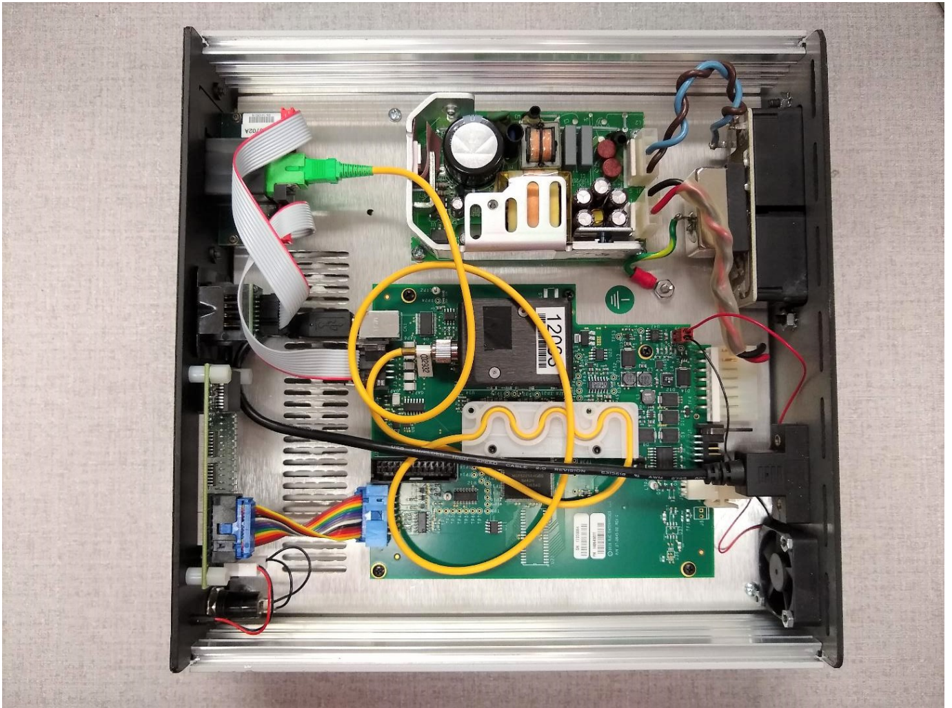
Figure 1: EUT Internal Photo Overview
