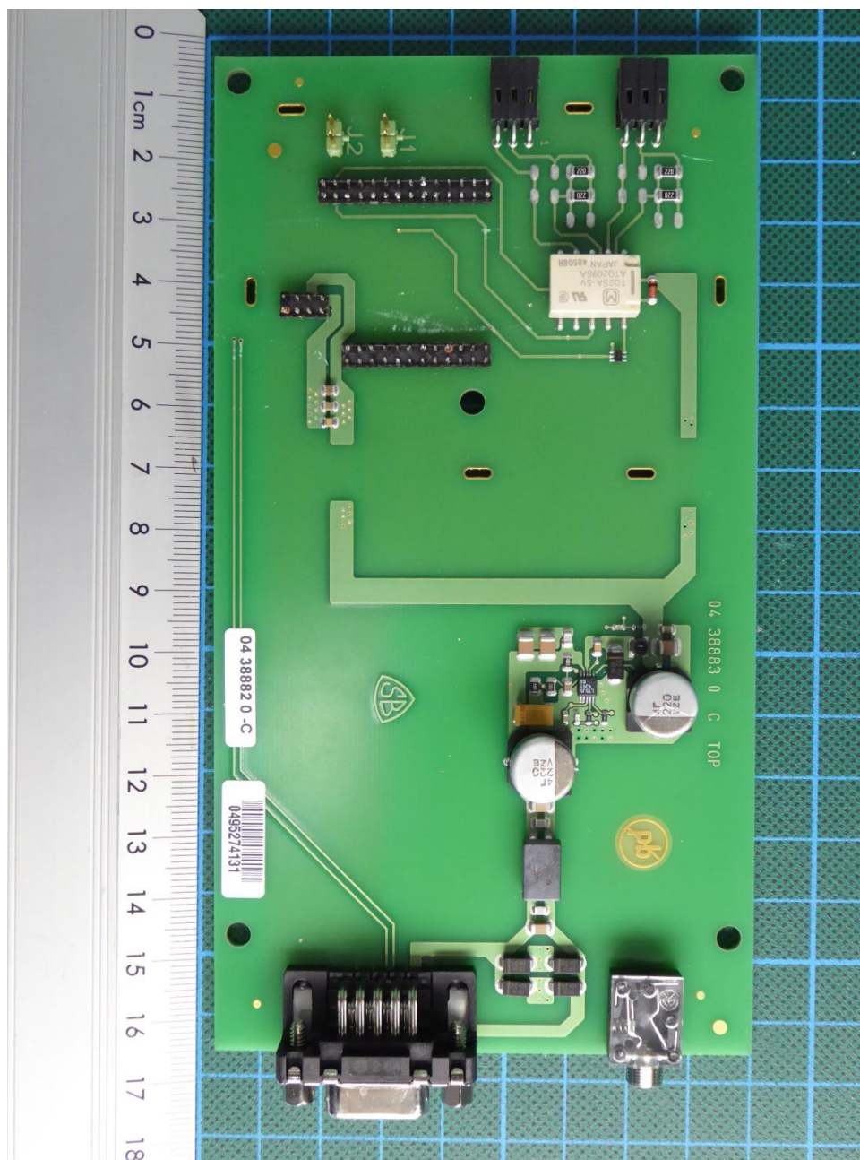
153615_19.JPG: EUT, top view, shielding and radio module removed
