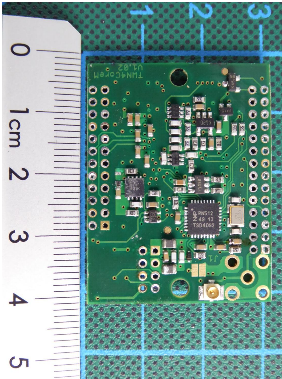
153615_21.JPG: EUT, radio module, bottom view
