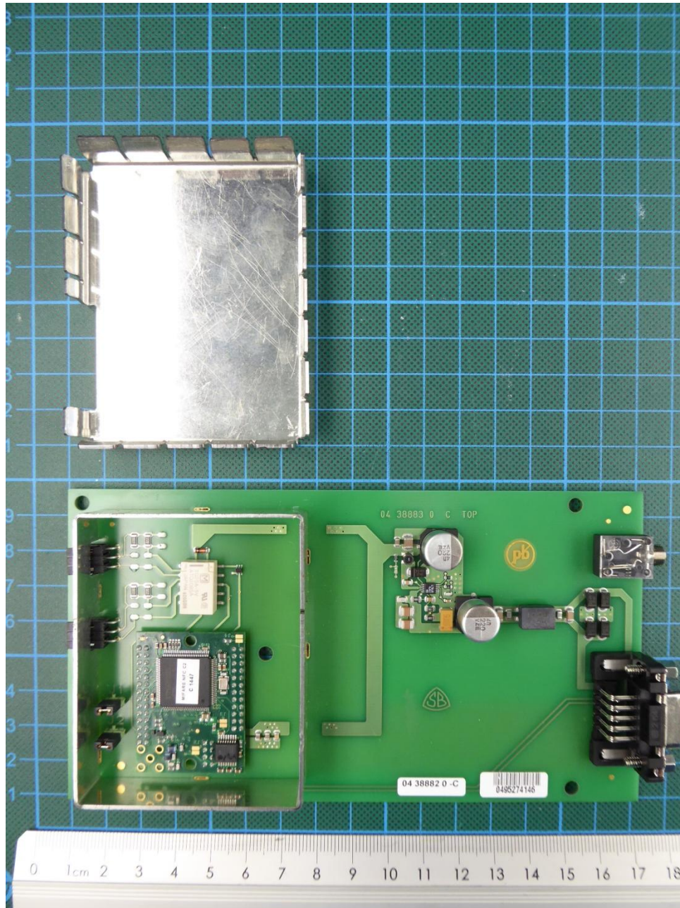
153615_18.JPG: EUT, top view, shielding removed
