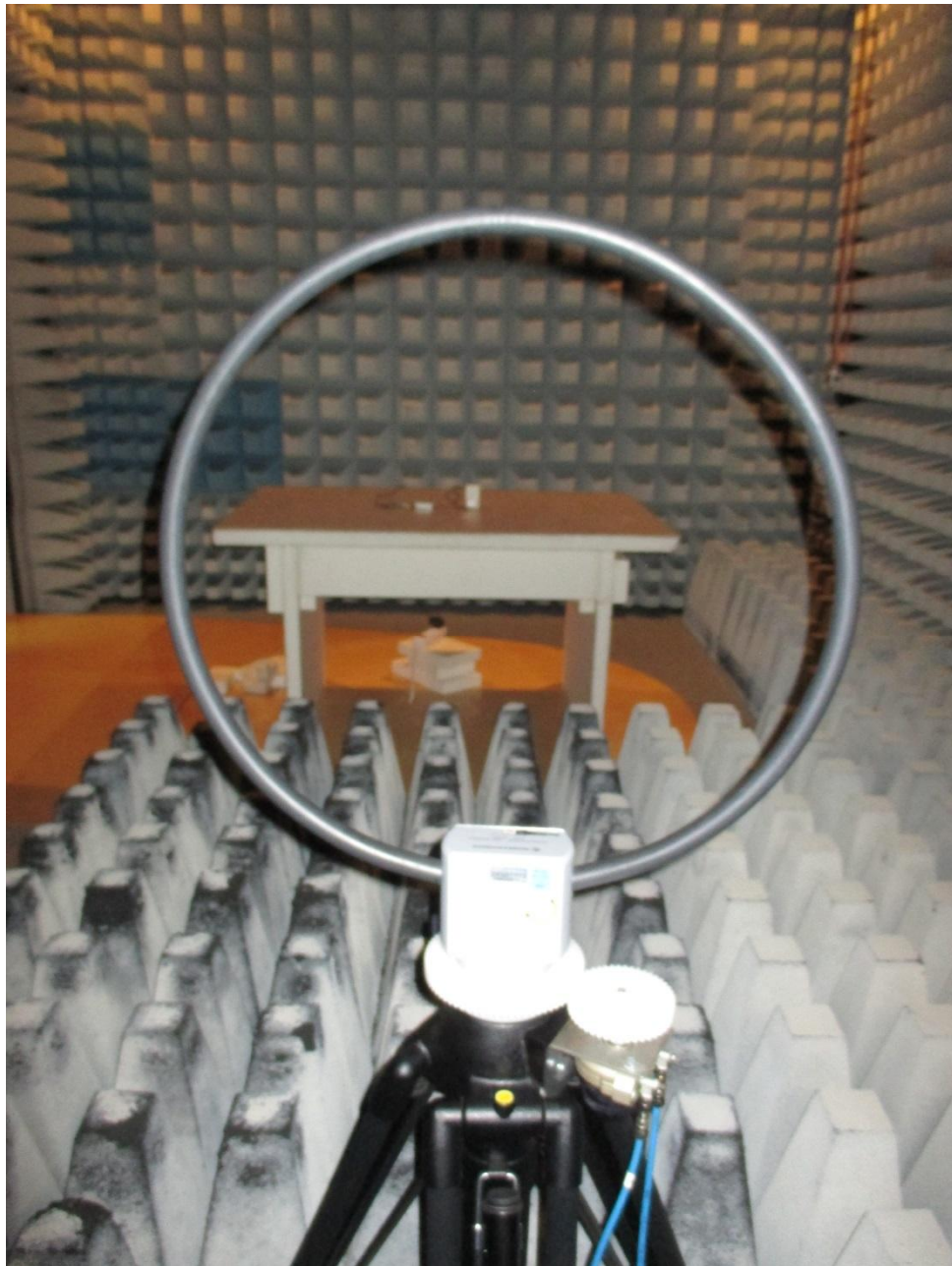
153615_1.JPG: Test setup anechoic chamber
