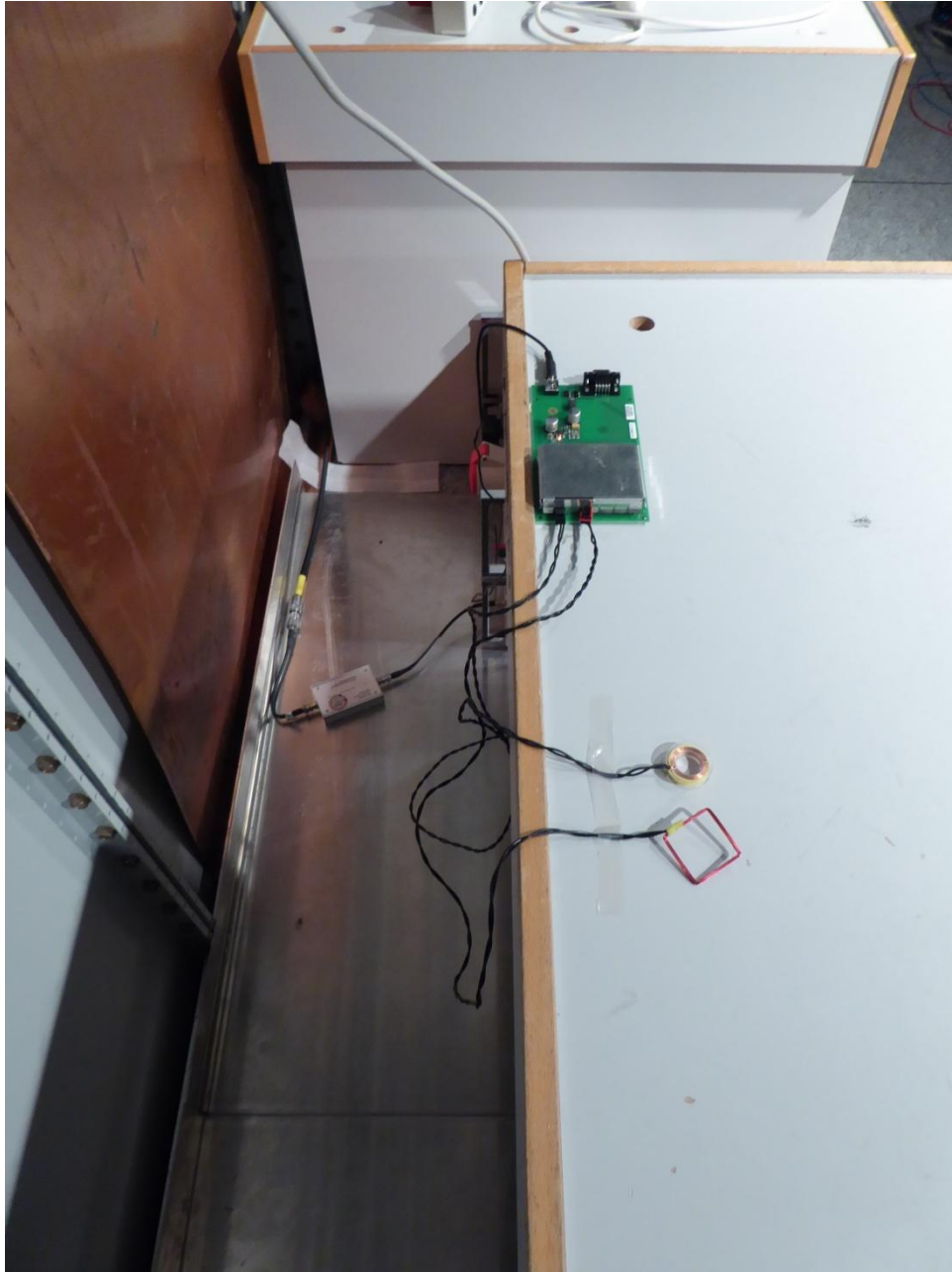
153615_5.JPG: Test setup conducted emission
