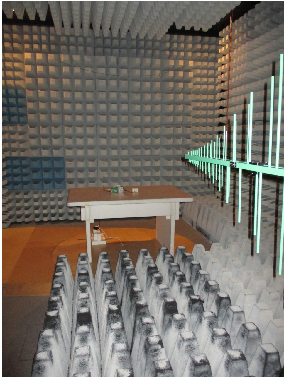
153615_2.JPG: Test setup anechoic chamber
