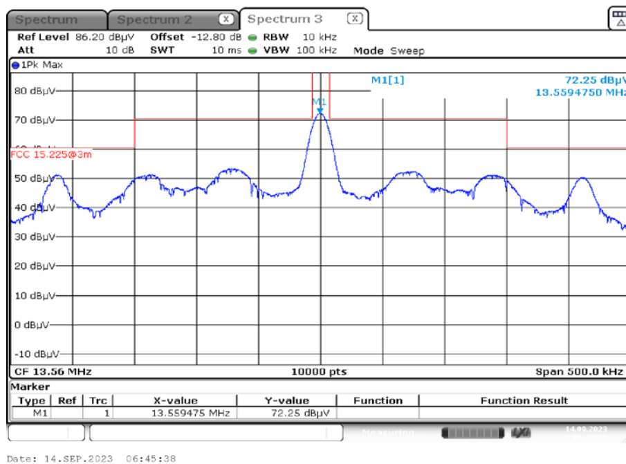
Plot 4: Spectrum mask – zoom
