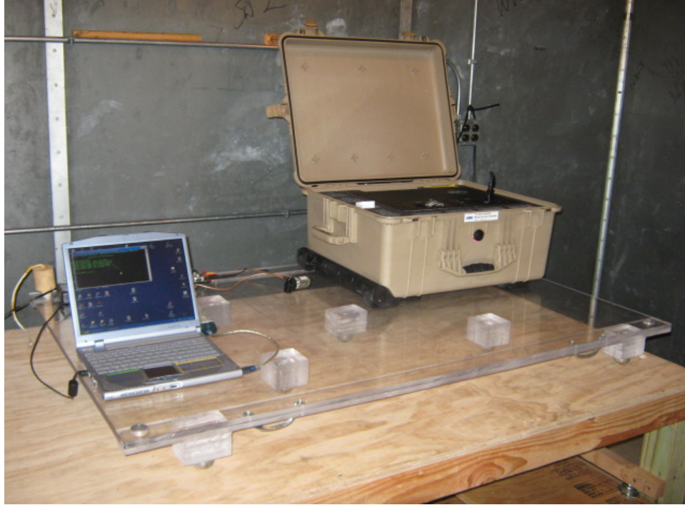
Mains Conducted Emission Test Table
