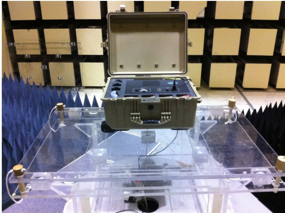
Radiated Spurious Tests
