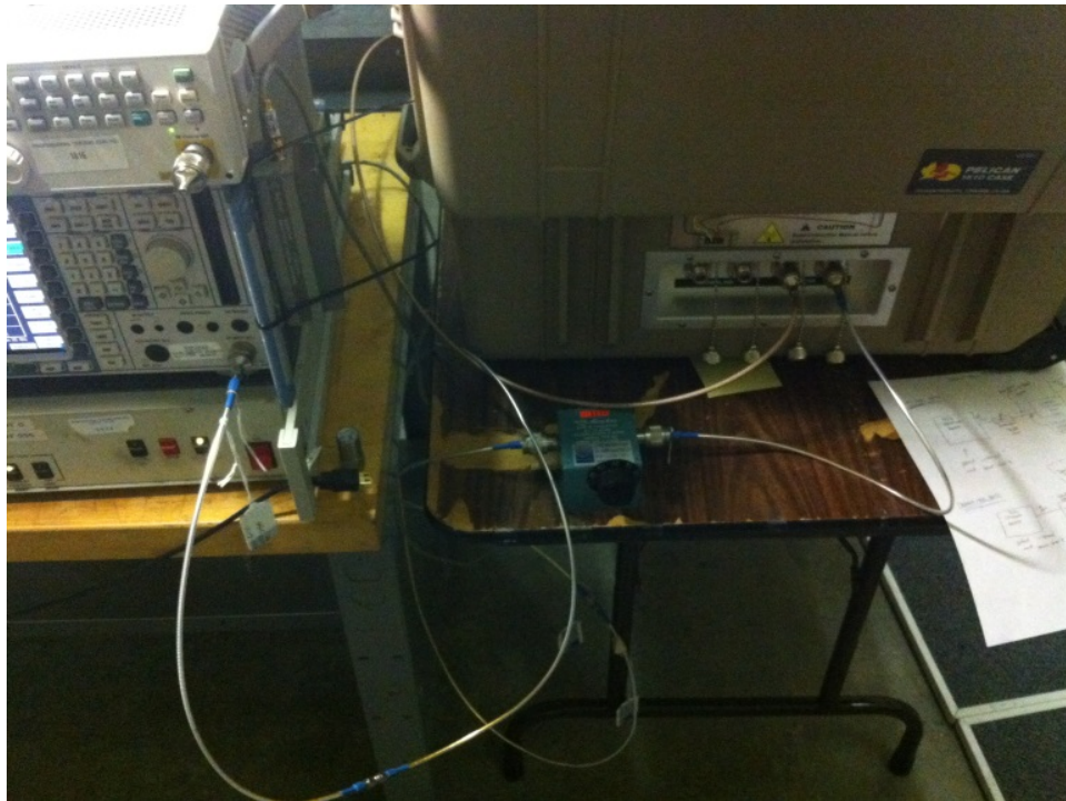
Conducted Output Tests (Power, BW, Spurious)
