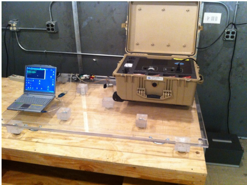
Mains Conducted Emission Test
