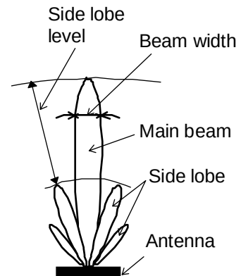
Fig.2-2 Antenna pattern
