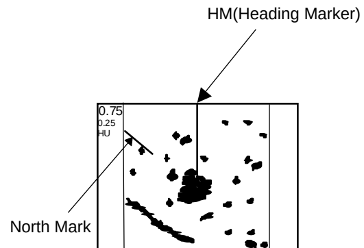
Fig.2-9 Heading Marker and North Mark
