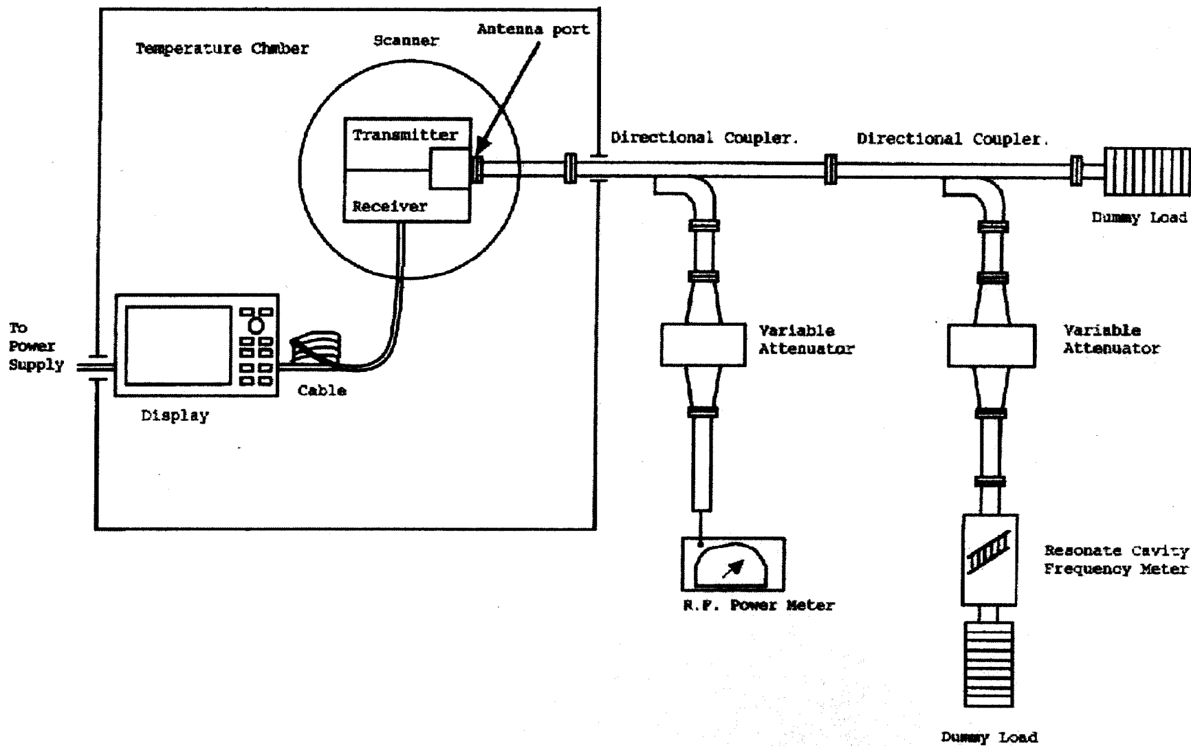
Figure 6 FREQUENCY STABILITY (2.985)
