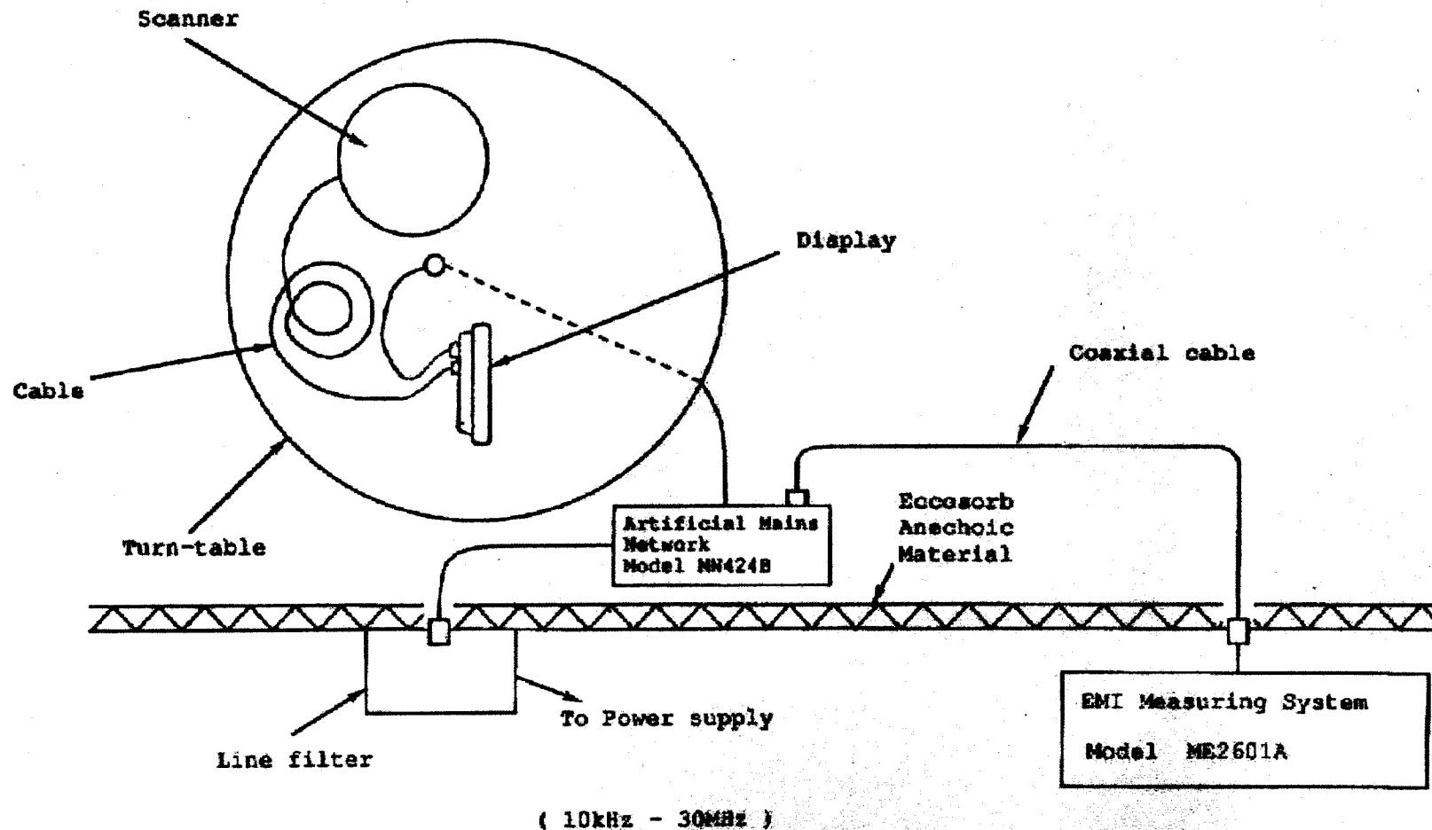
Spurious Emission Terminal Interference Voltage Figure 5
