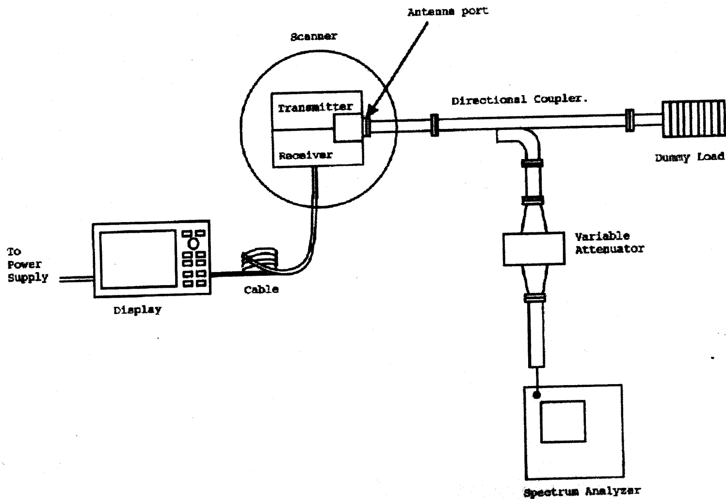
Figure 2 OCCUPIED BAND WIDTH(2.989) & SPURIOUS EMISSION AT ANTENNA TERMINAL(2.991)
