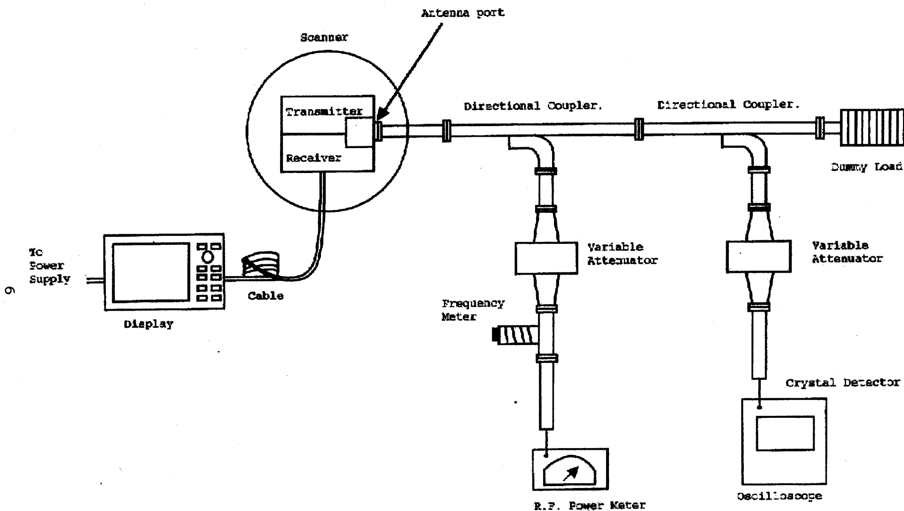
Figure 1 RF POWER OUTPUT & MODULATION CHARACTERISTICS(2.987)
