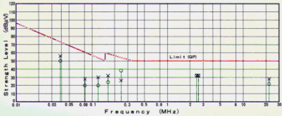
FIG 8 ***** Test Results of Conducted Power-Line Strength ***** per EN60945 (Frequency Range from 10kHz to 30MHz)
