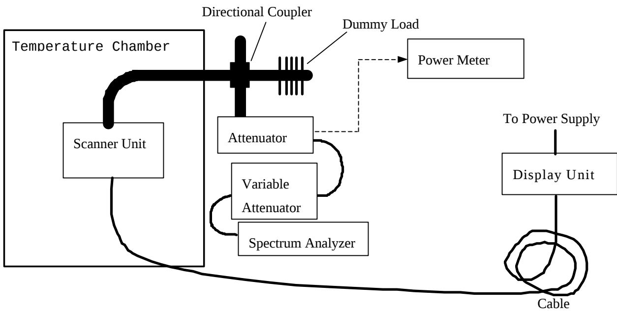
Figure.6 FREQUENCY STABILLITY (2.995)
