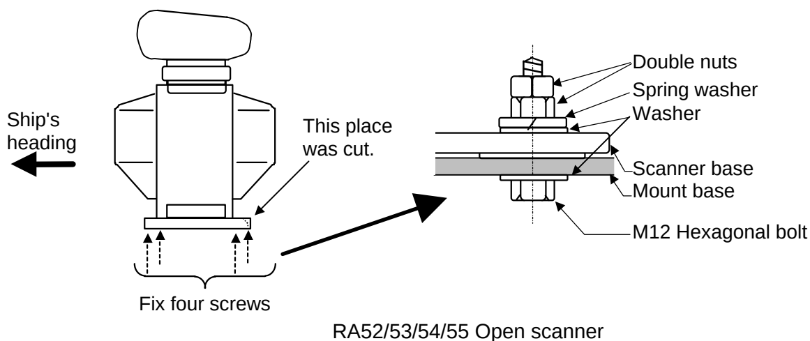
Fig.3-5 Mounting the Scanner
