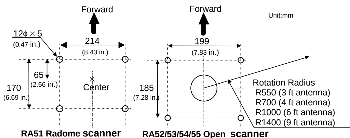
Fig.3-4 Hole positions for mounting scanner
