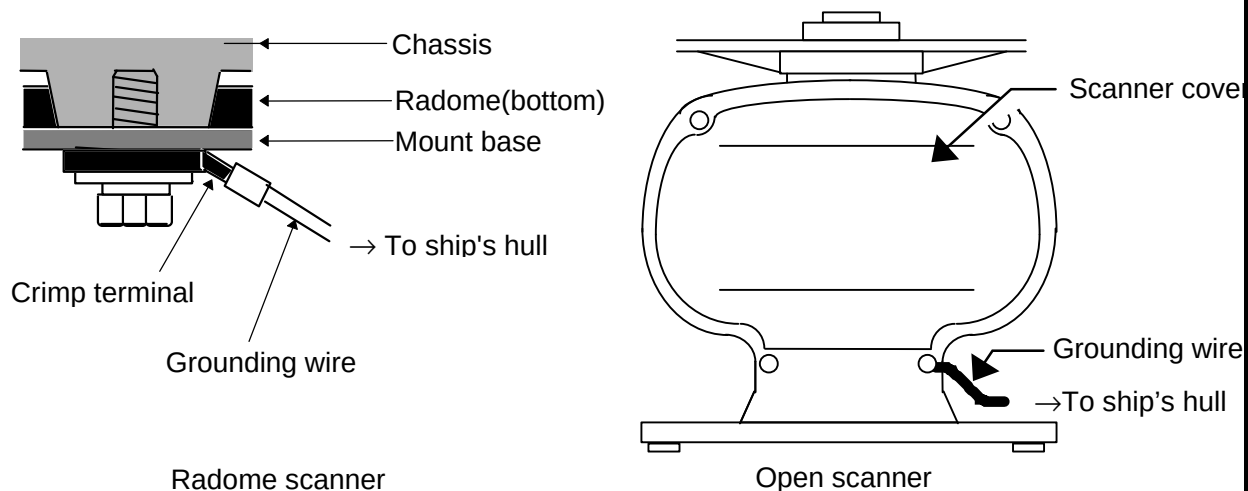
Fig.3-11 Grounding scanner unit to earth
