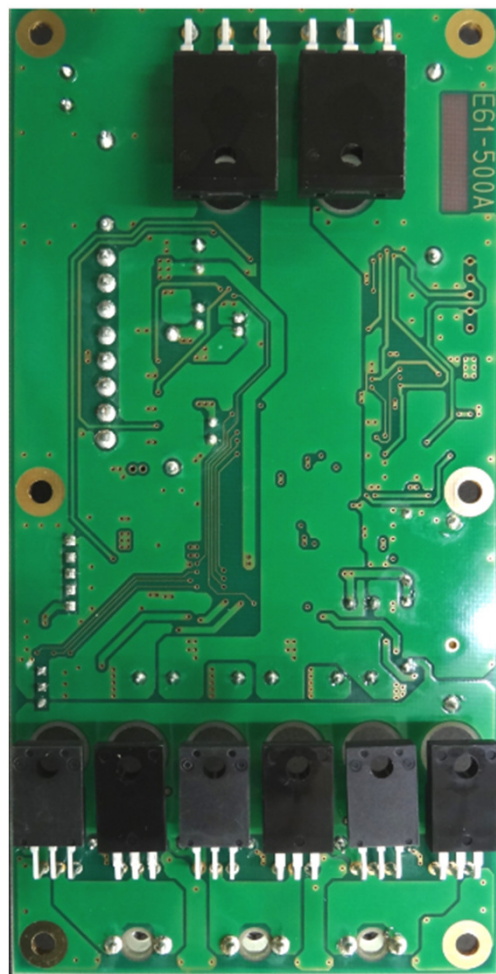
Bottom view
