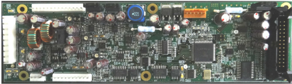
5.7 PCB: E61-120A Top view
