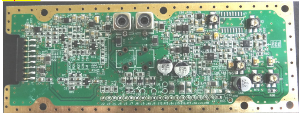
Bottom view
