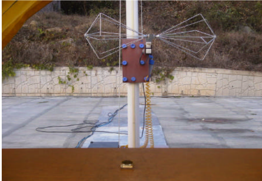
Photograph 1 : Setup for radiated Emissions
