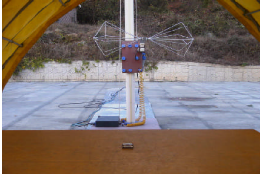
Photograph 1 : Setup for radiated Emissions
