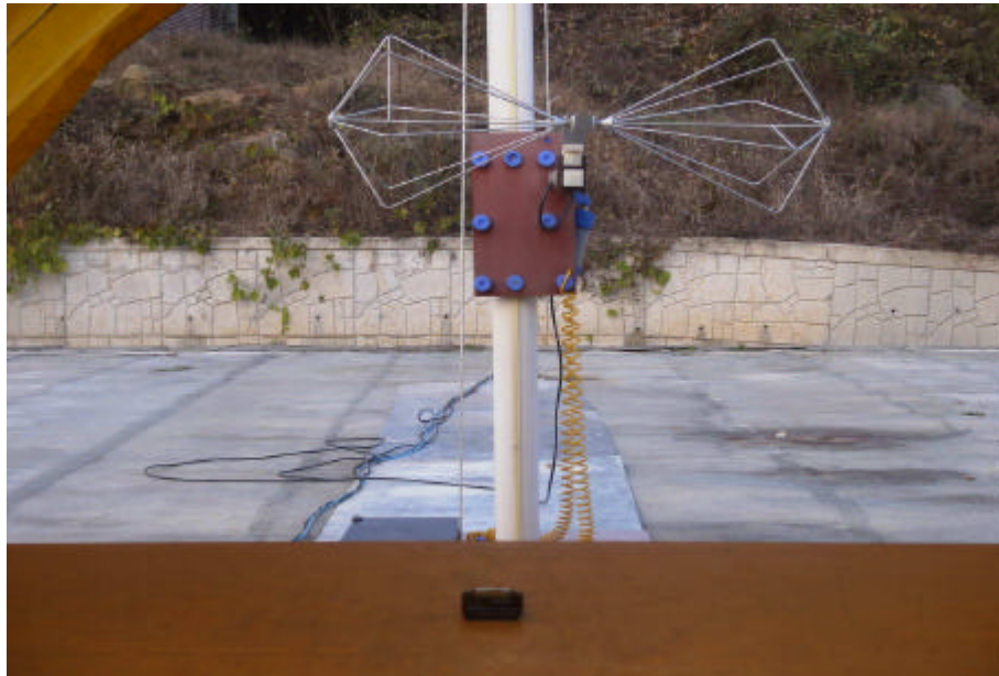
Photograph 1 : Setup for radiated Emissions
