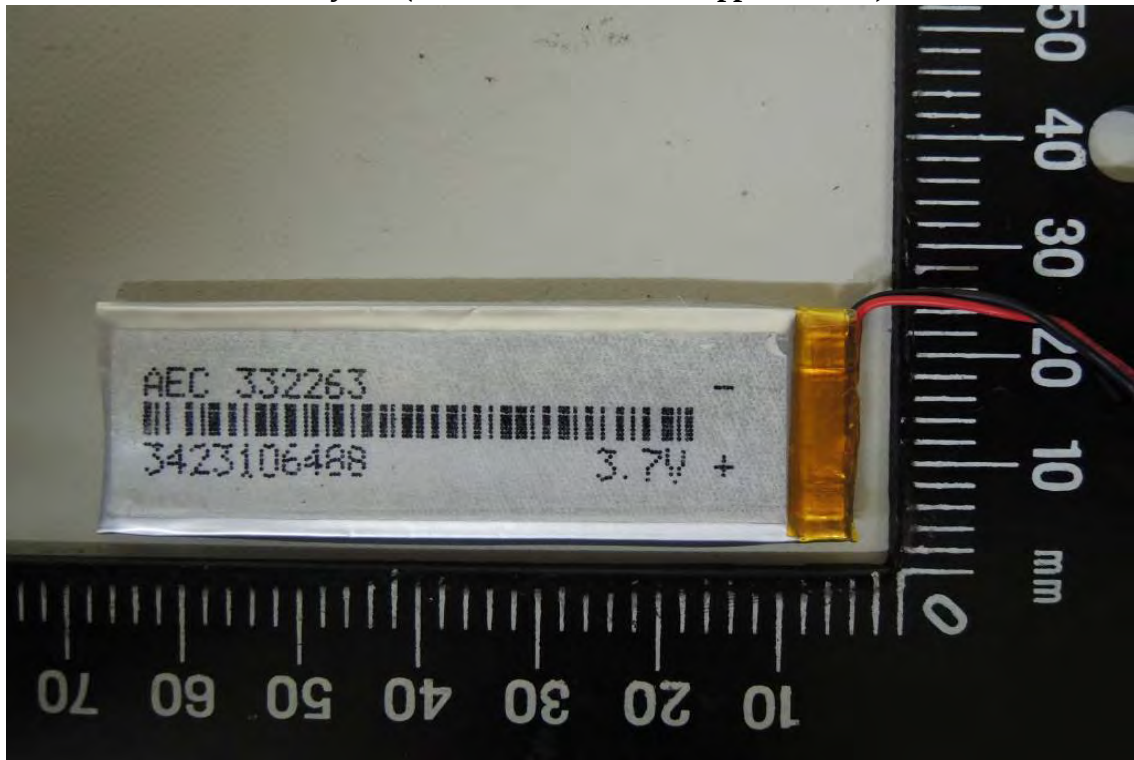
Battery – 2 (Model No.: 332263, Supplier: AEC)
