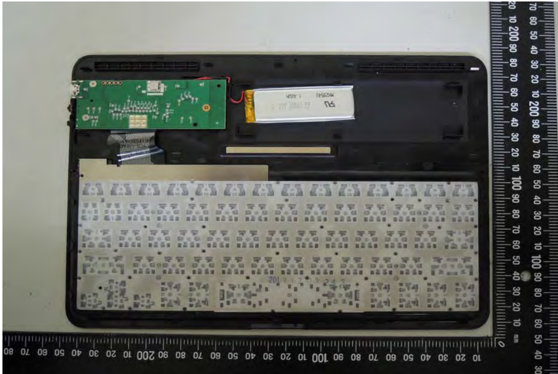
Open View of EUT-2(Non Backlight)
