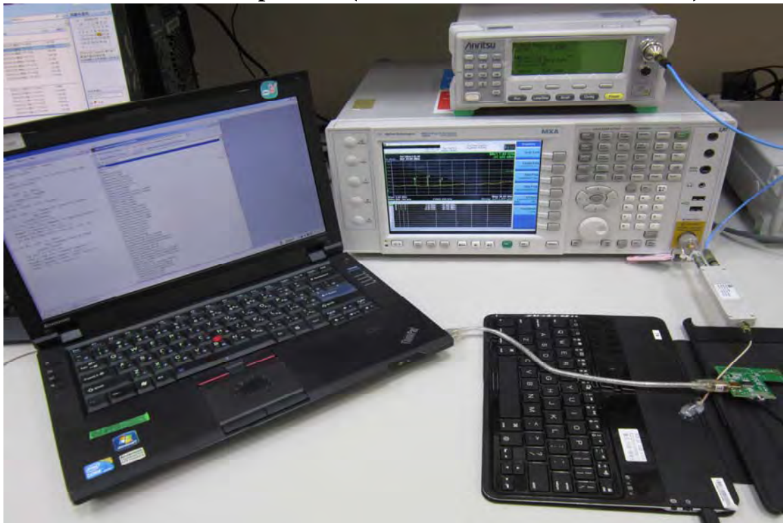
Conducted Setup Photo (Measurement at Antenna Port)
