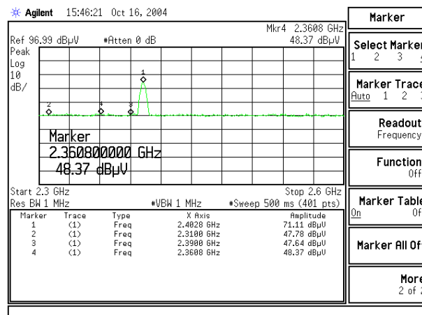
Figure Channel 00: (Vertical)
