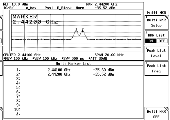
Channel 39 2441MHz
