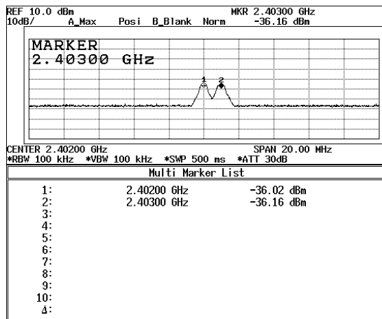
Channel 00 2402MHz
