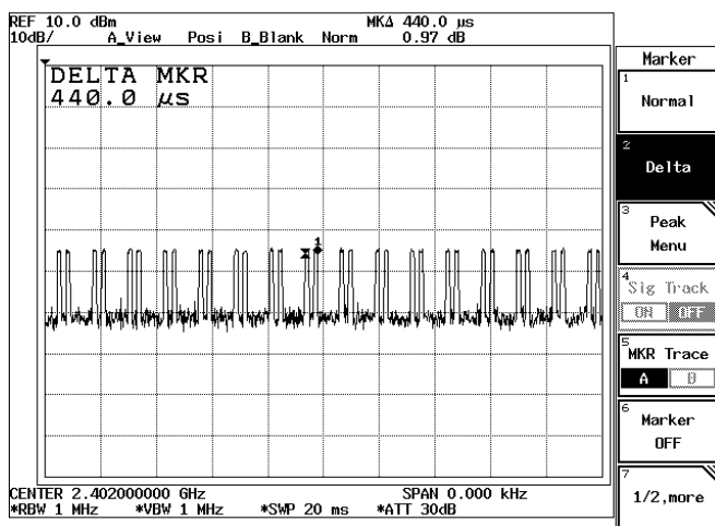
CH 00 2402MHz
