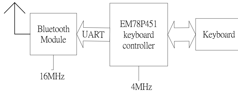
Fig.1 Keyboard Block Diagram
