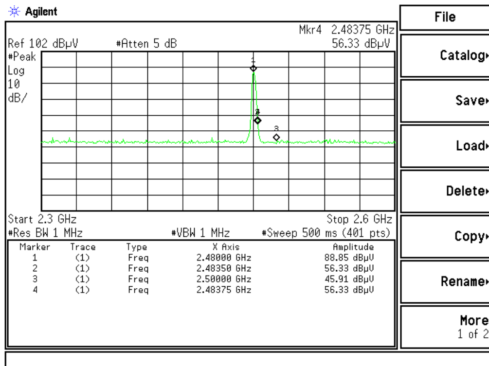
Figure Channel 78: (Vertical)
