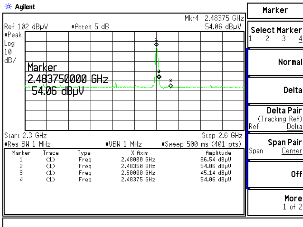
Figure Channel 78: (Horizontal)
