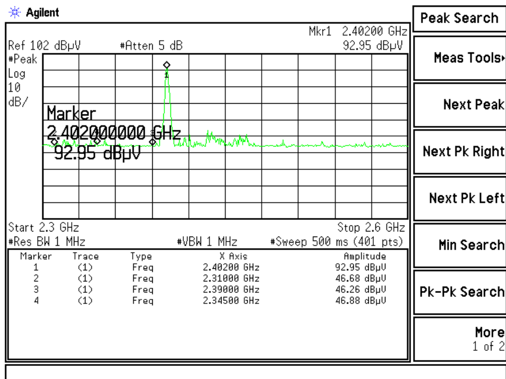
Figure Channel 00: (Vertical)
