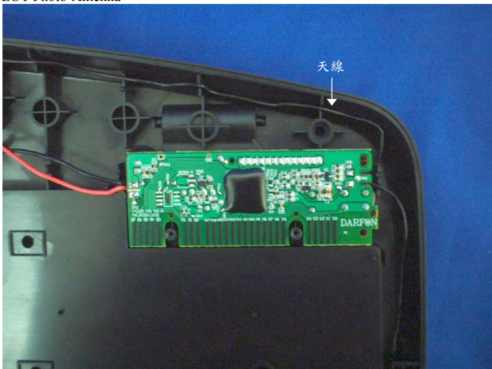
(4) EUT Photo-Antenna
