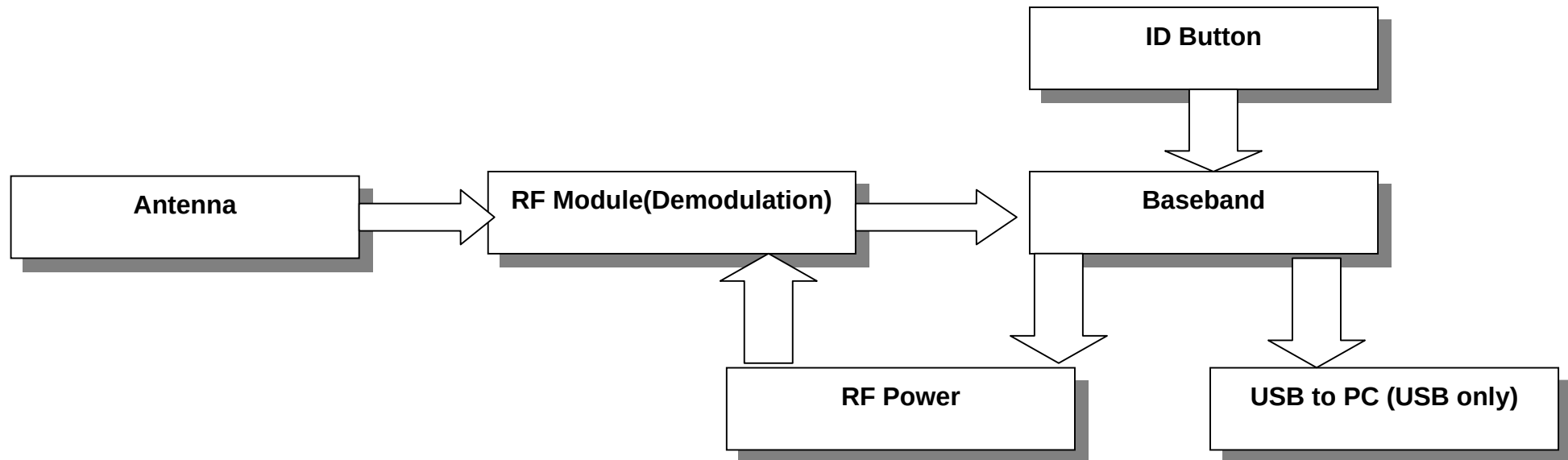
M310 Block Diagram
