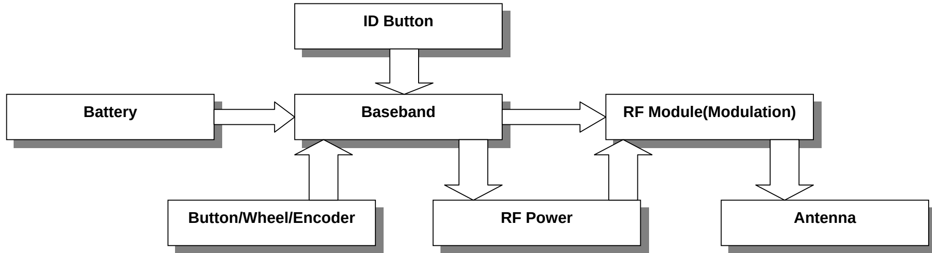
TX Block Diagram
