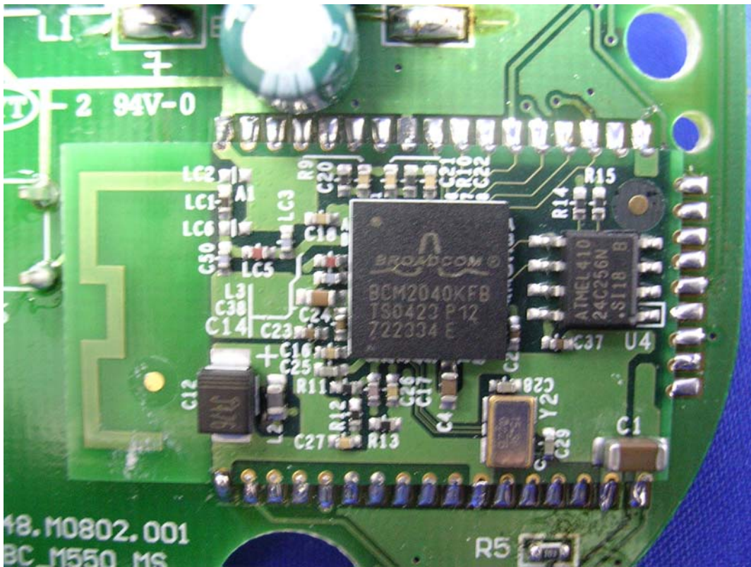
(7) EUT Photo
