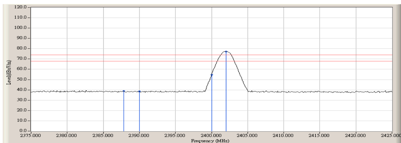
Figure Channel 00: (Horizontal)
