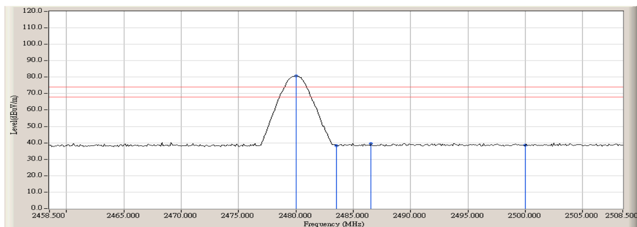
Figure Channel 78: (Horizontal)
