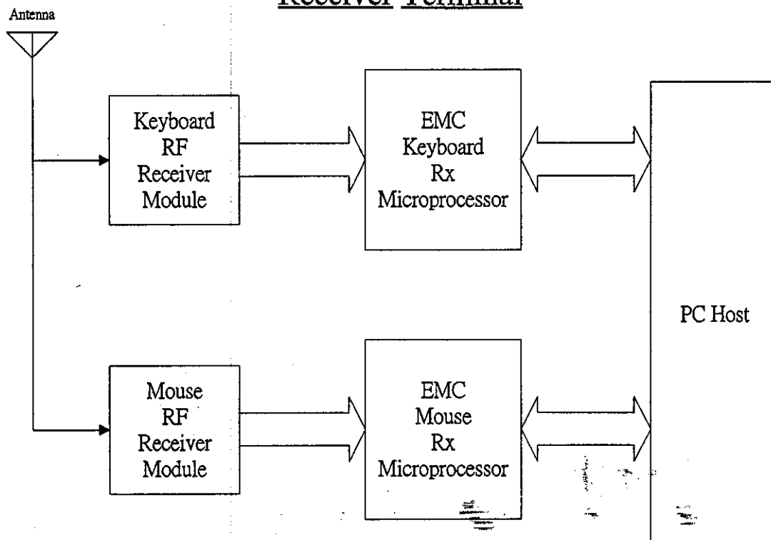
Fig.3 Receiver Block
