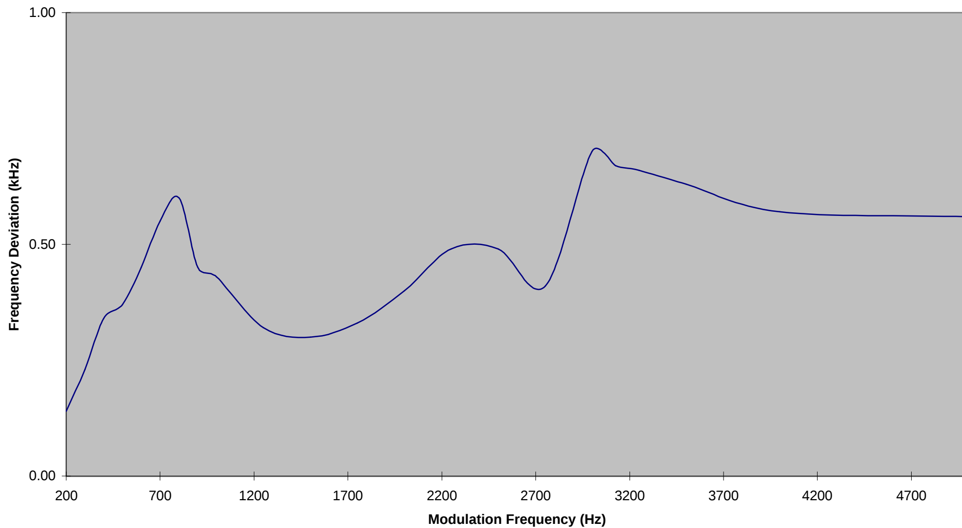
Modulation Frequency Response (Model: 1010)
